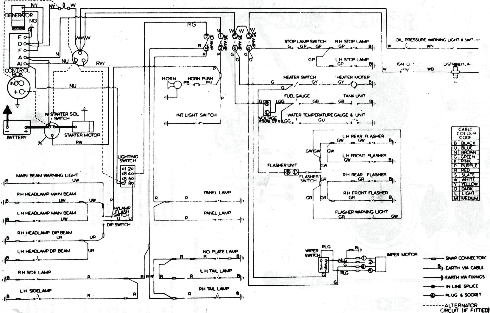
Rebel Circuit Diagram
